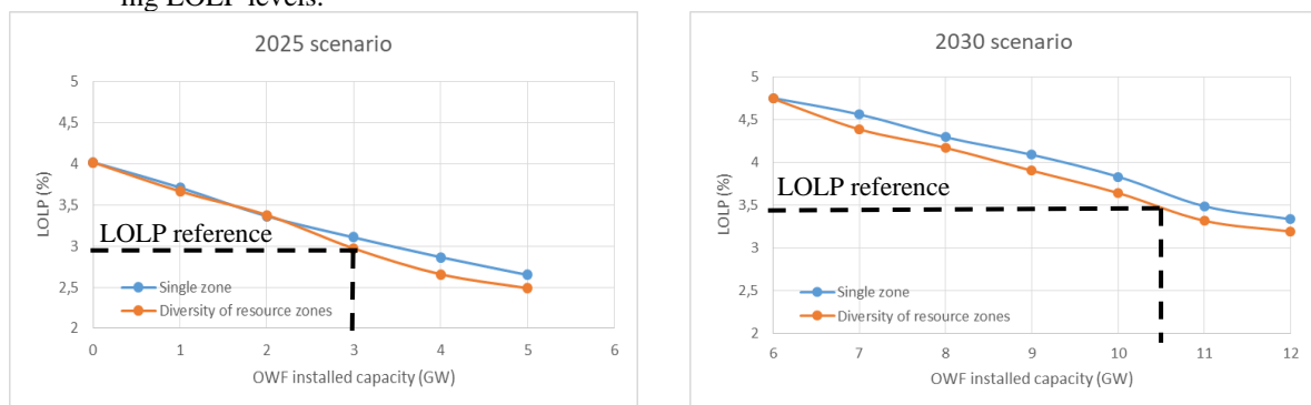
Fig. 2. Impact of offshore wind capacity to the Loss of Load Probability
