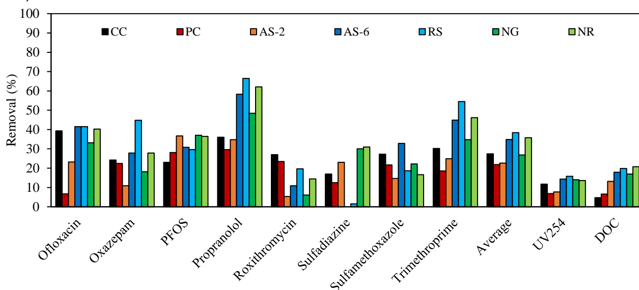
Figure 2. OMPs, UV 254 , DOC removals and average OMPs removal for the 7 μGACs studied (10 mg/L, crushed and sieved at 50-63 μm, initial UV 254 = 0.204 1/cm and initial DOC = 10.6 mgC/L) after 30 min of contact time with nitrified water.
