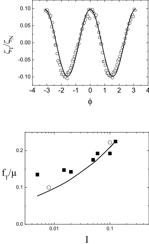
FIG. 15: Angular distribution of tangential contact forces: (a) \zeta_T(\phi)/\zeta_N(\phi) ( \circ ) fitted by f_T \cos(2\phi) (—) for I = 0.13 and \mu = 0.4 , (b) f_T(I)/\mu for \mu = 0.4 ( \circ ) and \mu = 0.8 ( \blacksquare ) compared with \frac{\sqrt{2}}{\pi}I^{1/3} .
