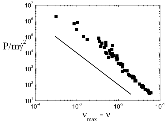
FIG. 4: P/\dot{\gamma}^2 as a function of (\nu_{max} - \nu) . The straight line indicates a slope of -2 ( \mu = 0.4 , various e ).
