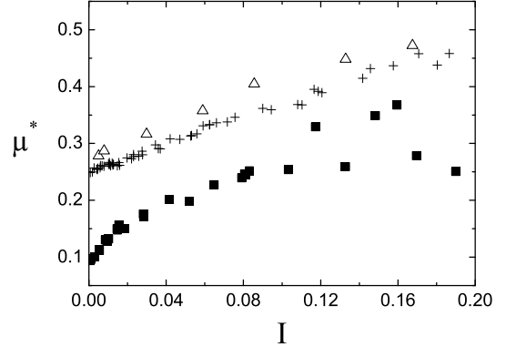
FIG. 6: Influence of \mu on the friction law ( \mu = 0 (■), \mu = 0.4 (+), \mu = 0.8 (Δ), various e ).
