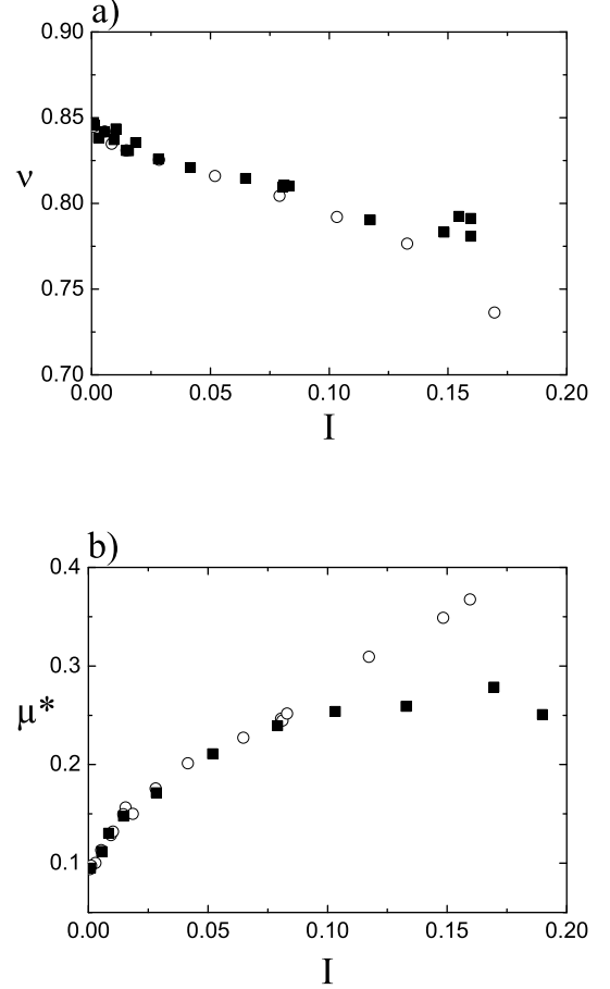
FIG. 8: Influence of e for \mu = 0 ( e = 0.9 (■), e = 0.1 (○)) : (a) Dilatancy law, (b) Friction law.
