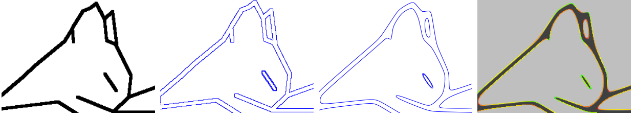
Figure 8: Detail of Attneave's cat (a binary image, see Figure 1), level lines (at quantization q = 200 ) before and after smoothing (scale t = 5 ) and curvature map.
