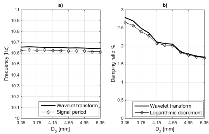
Figure 6 – a) TMD's damped frequency and b) TMD's damping ratio for fixed D_1 = 0.24 \text{ mm} and varying D_2
