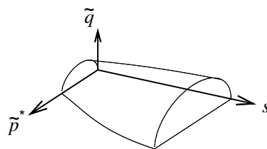
Fig. 5 Form of the yield surface in the (\bar{p}^*, s, \tilde{q}) plane
