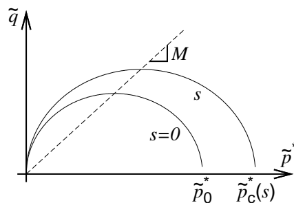
Fig. 4 Yield surface in the (\bar{p}^*, \tilde{q}) plane
