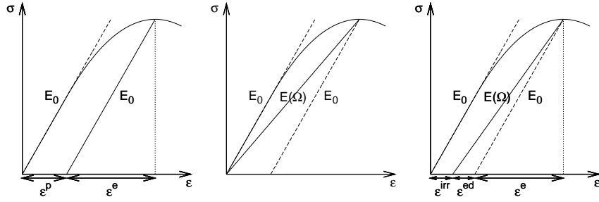
Fig. 1 Plastic behaviour
