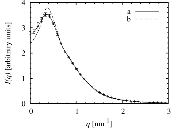
FIG. 14. The average blurred spectrum I_w(q) (a) of configurations poly030 , poly036 , poly042 , poly048 ( \alpha = 0.51 ), and the resulting deblurred spectrum I(q) (b).
