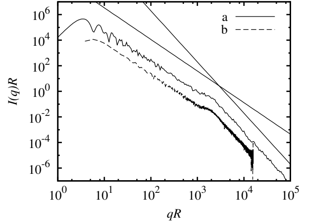
FIG. 19. Scattered intensity pattern of the Apollonian packing shown in figure 18, computed with the method proposed in this paper (a), and with the approximate formula (33) (b). The two curves are in excellent agreement, and match perfectly without rescaling; for the sake of readability, curve (b) has been translated vertically. The two straight lines represent the expected fractal ( I(q) \propto q^{-2.47} , low q ), and Porod ( I(q) \propto q^{-4} , high q ) regimes. In order to allow for the direct comparison of the two methods, both q and I(q) have been made dimensionless through multiplication by the external radius R of the packing; furthermore, \Delta \rho = 10^{10} R^{-2} .
