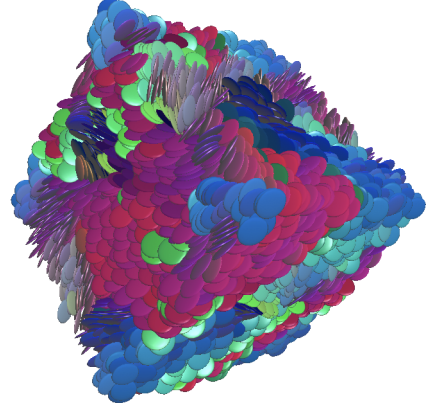
FIG. 9. An example of dense packing of oblate spheroids generated following the procedure described in section IV A. The radii of the particles are a = 200 (equatorial radius), c = 25 (polar radius). The total number of particles is N = 10000 , the compacity is 60 %. [Color online] Each particle is colored according to its orientation, which emphasizes the fact that high compacity causes local orientational order.
