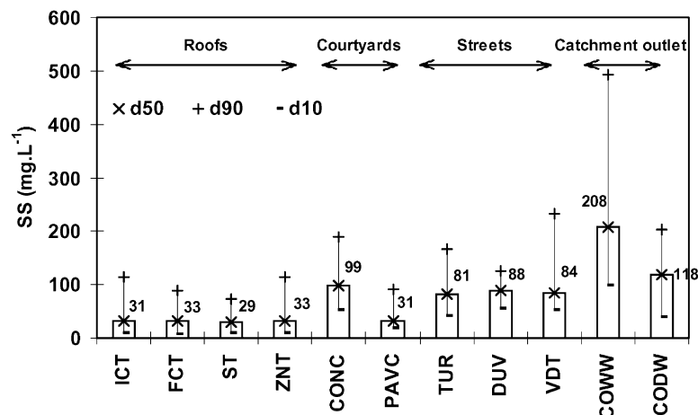
Fig. 2. Suspended solid (SS) concentration (mg L -1 ) in the samples from the “Le Marais” experimental urban catchment (figures give the median value).
