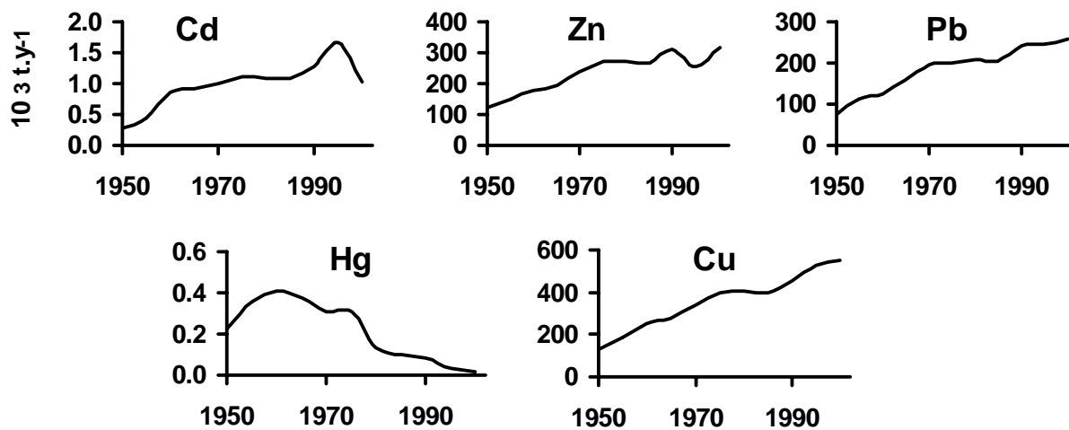
Figure 8: Total annual metal demand from industries in France ( \text{t.y}^{-1} ) (Lestel, in preparation)
