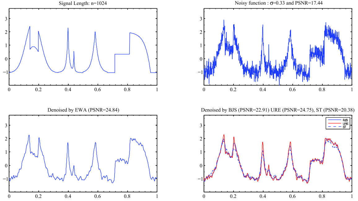
FIG 5. This figure presents the results of signal denoising for function Piece-Regular. The first row is the true signal (left) and a noisy version of it (right), where the noise is white Gaussian with standard deviation \sigma = 0.33 . The second row presents the denoised signals obtained by EWA (left) and by BJS, ST and URE (right)
